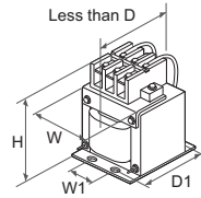
FR-HEL-3.7K to 30K FR-HEL-H0.75K to H30K
