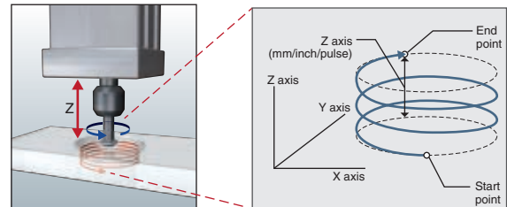
Helical interpolation *1
