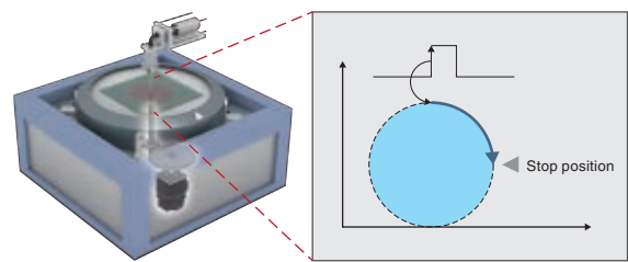
Speed-position switching *1
