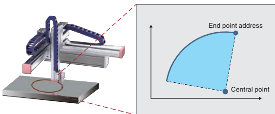
Circular interpolation
